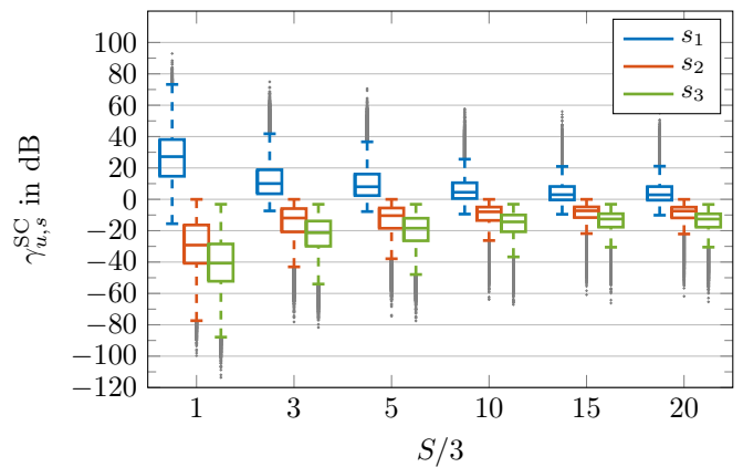
Figure 1: SINR to the three strongest SeNBs, denoted as s_1, s_2, s_3 , for different numbers of SeNBs per sector.
