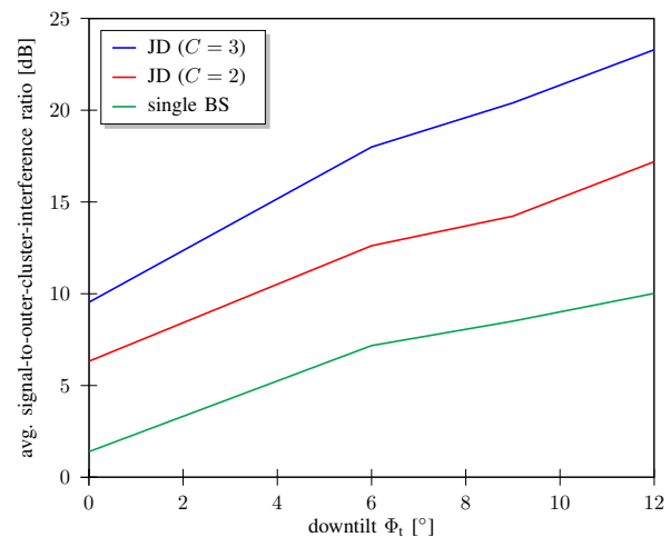
Fig. 5. Average SOCIR using JD of either 2 or 3 BSs
