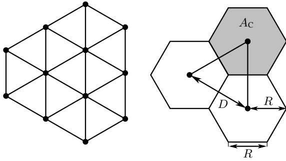
Fig. 1: Regular grid of macro sites and corresponding cell geometry with D = \sqrt{3}R and A_C = \frac{3\sqrt{3}}{2}R^2 .
