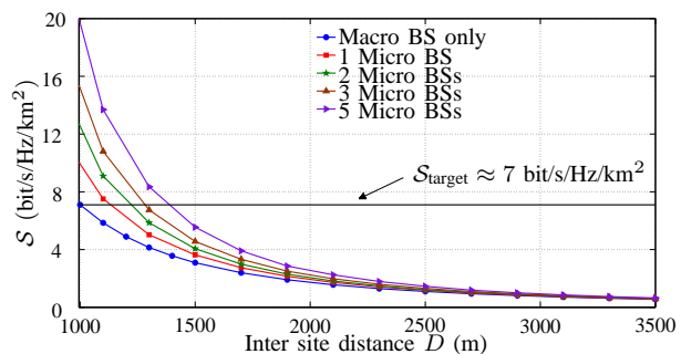
Fig. 4: Area spectral efficiency as function of inter site distance for different deployments
